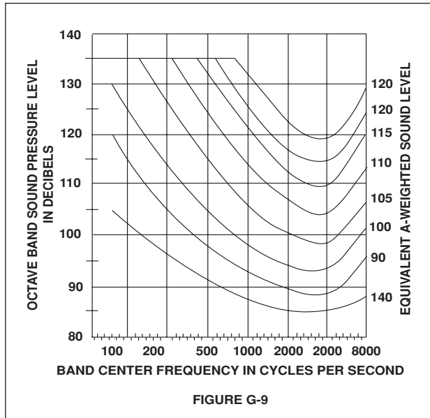
FIGURE G-9 – Equivalent A-Weighted Sound Level. Equivalent sound level contours. Octave band sound pressure levels may be converted to the equivalent A-weighted sound level by plotting them on this graph and noting the A-weighted sound level corresponding to the point of highest penetration into the sound level contours. This equivalent A-weighted sound level, which may differ from the actual A-weighted sound level of the noise, is used to determine exposure limits from Table 1.G-16.
